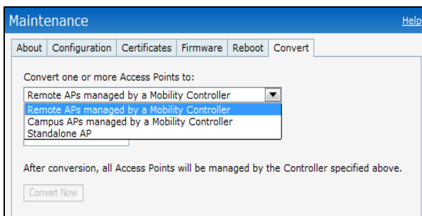
Figure 97 - Convert options
