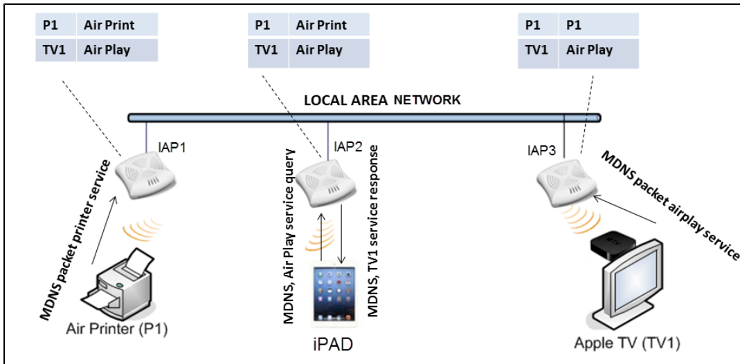
Figure 89 - AirGroup Architecture
