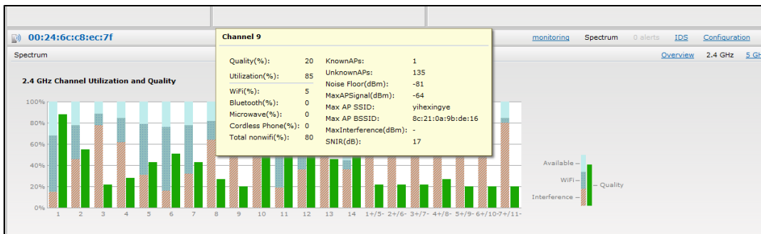
Figure 60 Channel Details
