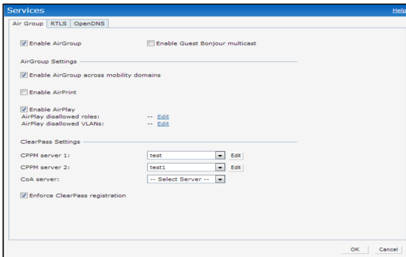
Figure 92 AirGroup Configuration
