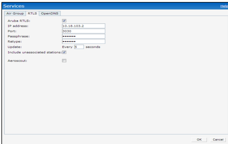
Figure 93 RTLS Window
