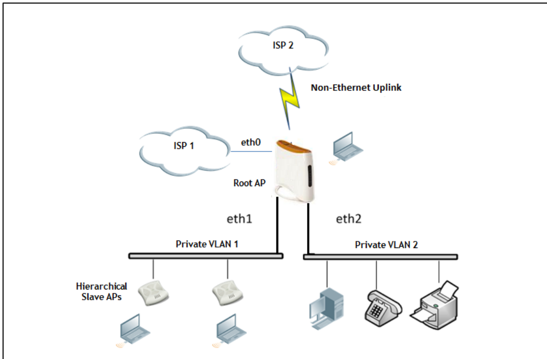
Figure 37 Hierarchical Deployment
