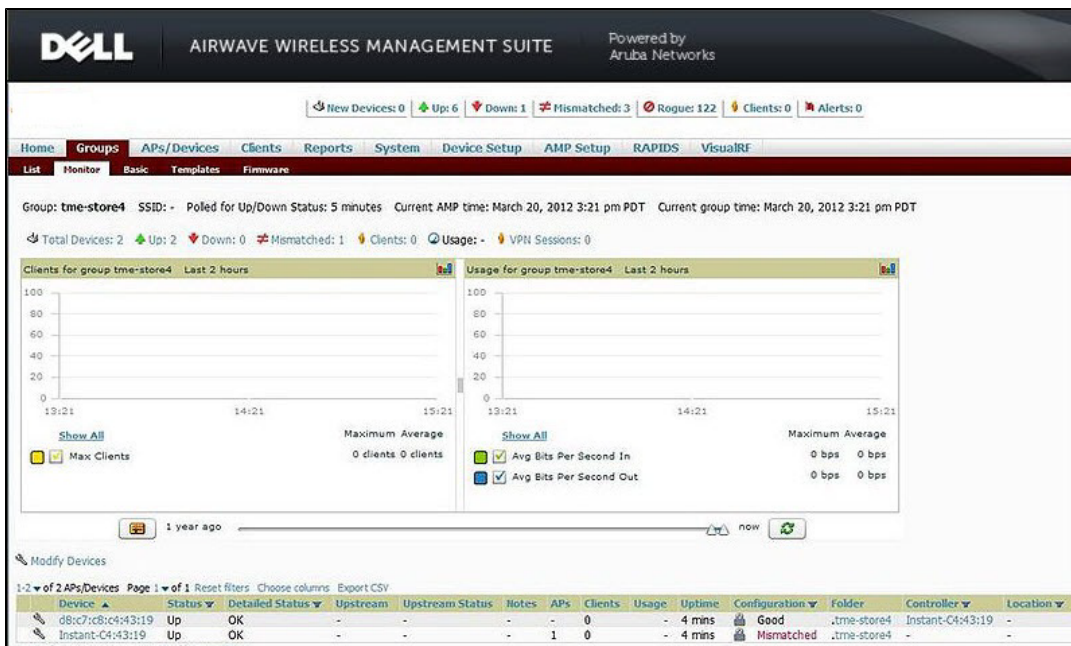
Figure 88 W-AirWave — Monitor
