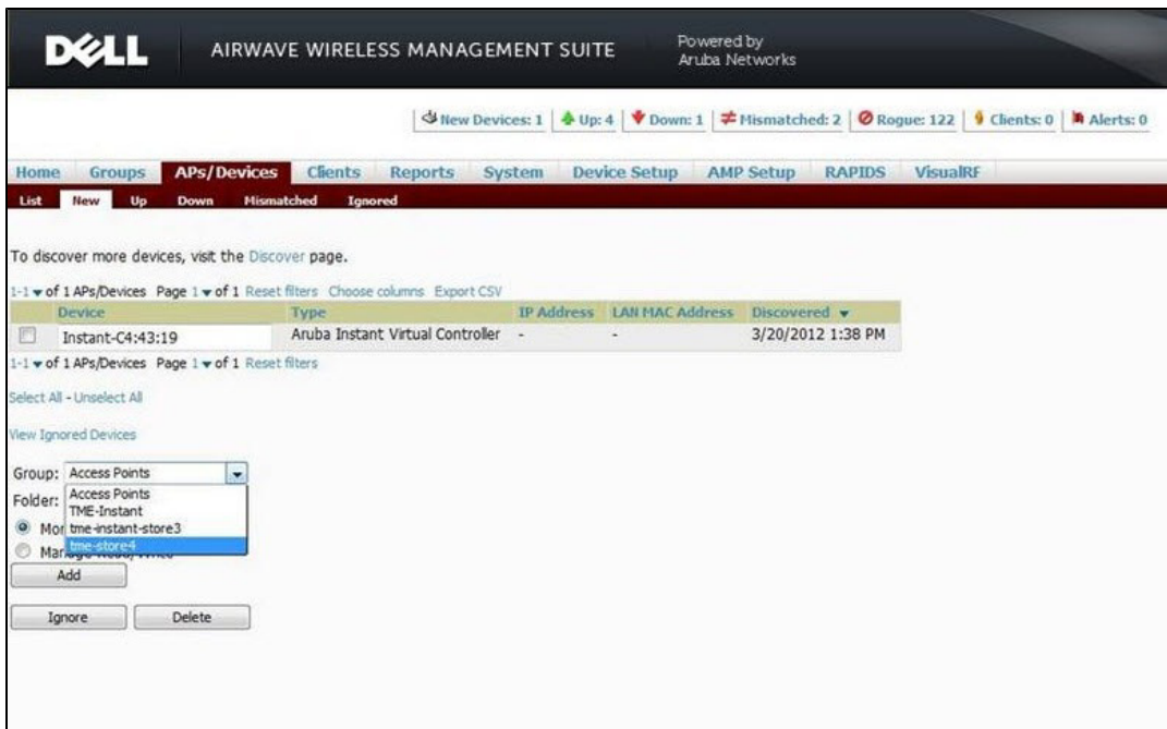
Figure 88 W-AirWave — Monitor
