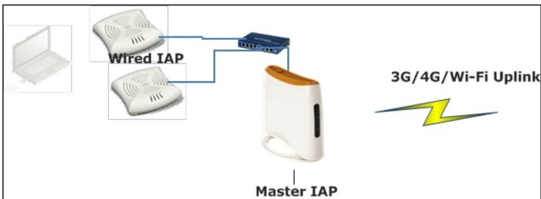
Figure 34 Uplink Types
