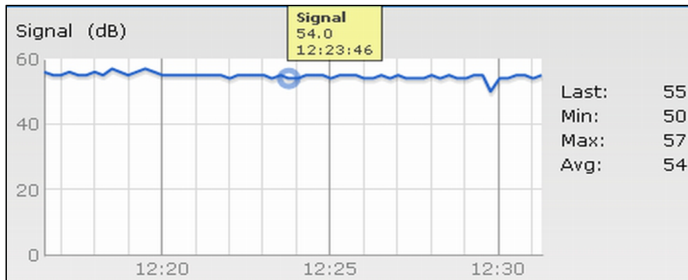
Figure 17 Frames Graph
