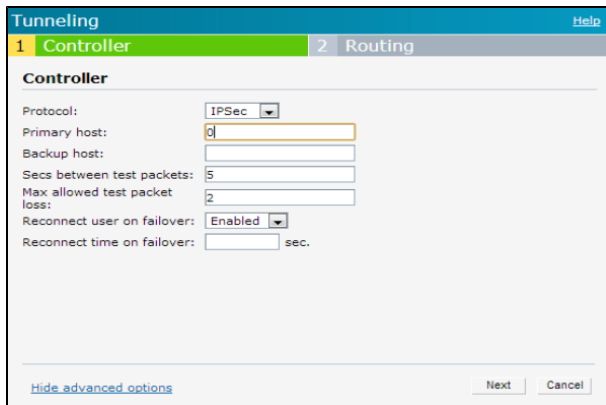
Figure 71 IPsec Configuration
